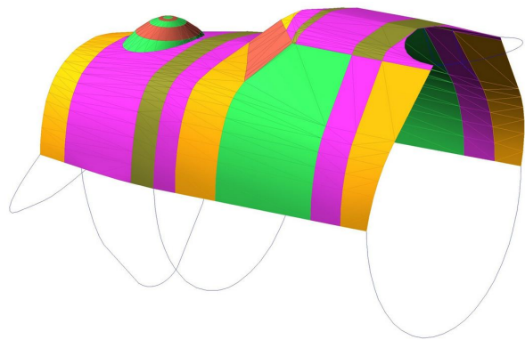
Boeing B-17 Extended Canopy Cover, 3D model
